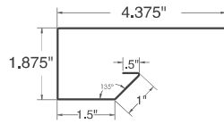
PERIMETER G-CHANNEL
