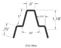
PANEL CARRIER
