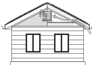
The gable-louver vent, an exhaust vent, allows unwanted air to flow out of the attic.
